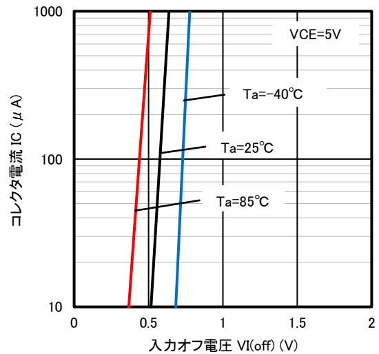
入力オフ電圧 V_i(off) (V)
